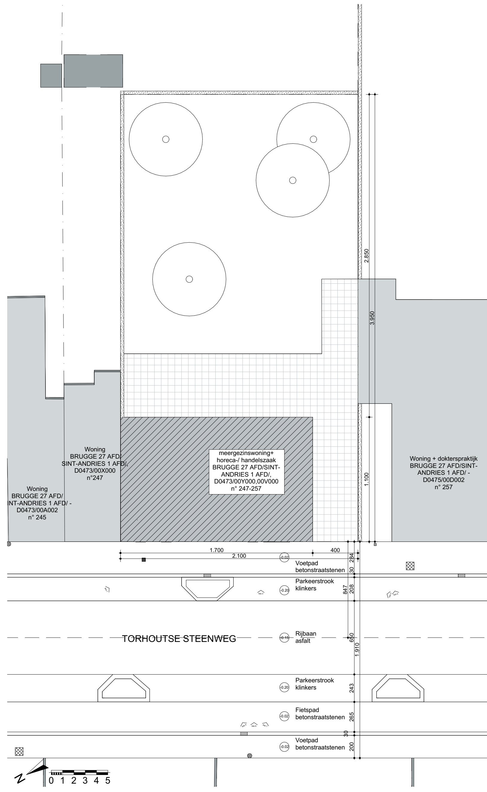
0.2 inplantingsplan NT 1:200
